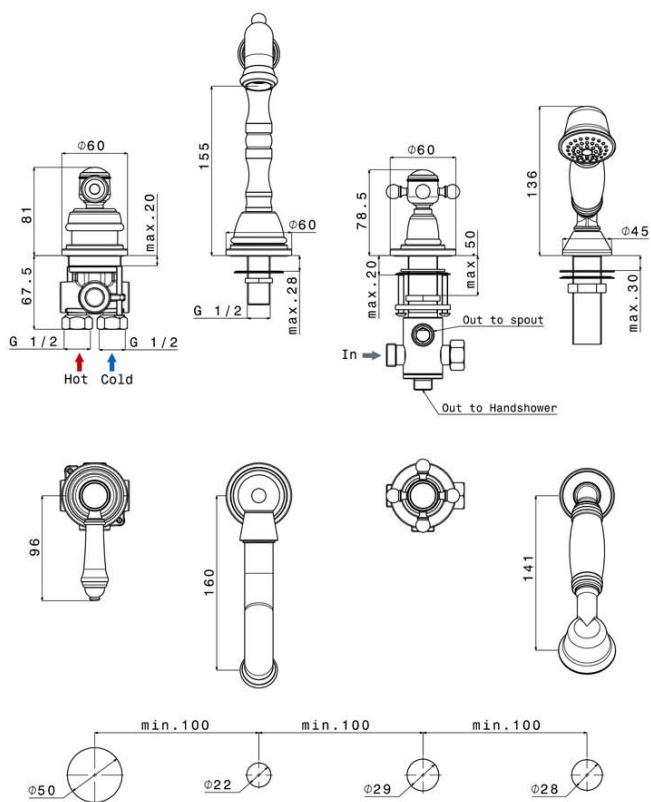
Installation holes
