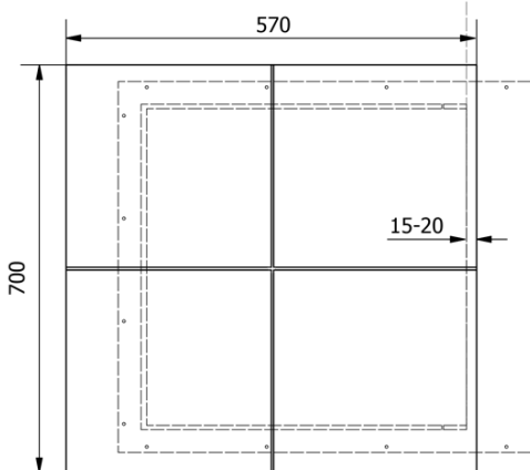
Maximum tiling
